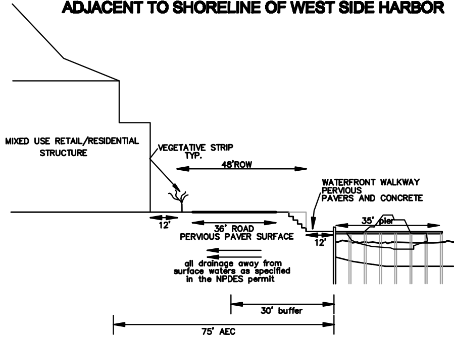
GENERALIZED CROSS-SECTION OF THE ESPLANADE AREA
