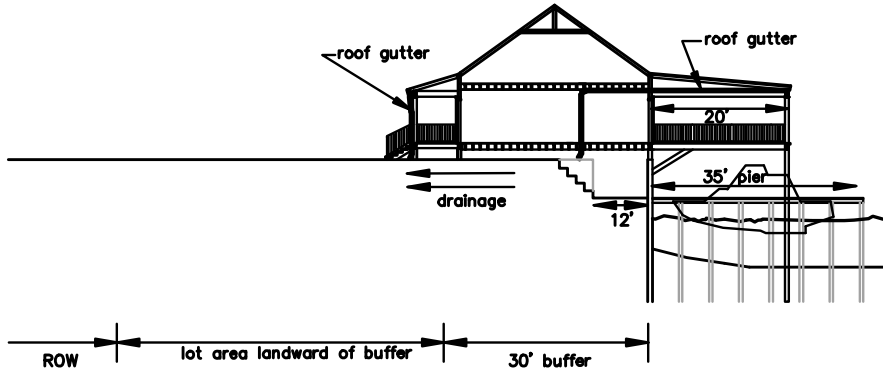
CROSS-SECTION WITH 20' PORCH OVER THE WEST SIDE HARBOR
