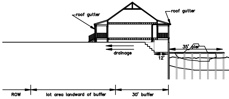
GENERALIZED CROSS-SECTION ADJACENT TO SHORELINE OF WEST SIDE HARBOR
